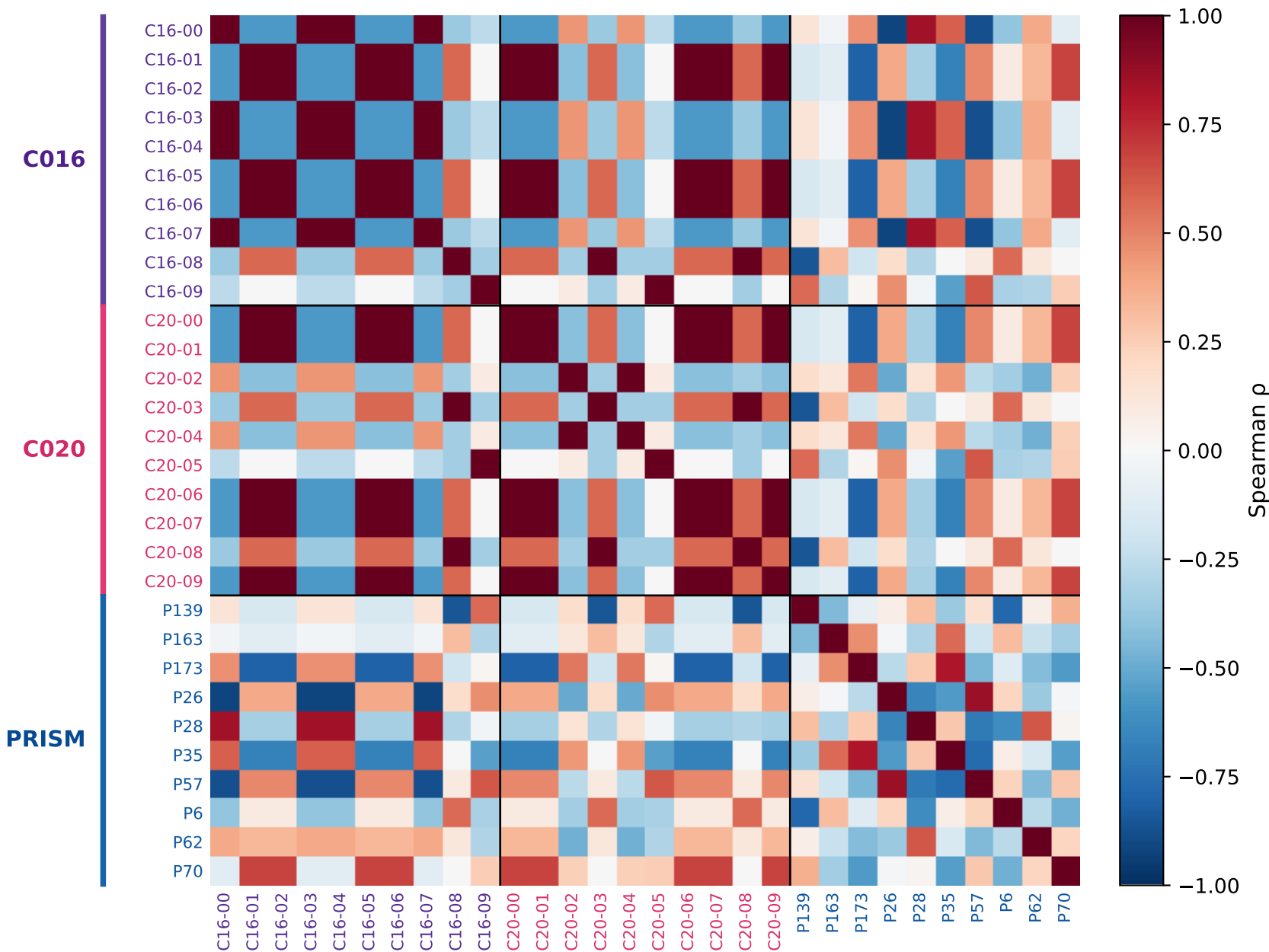
Pairwise jury rank agreement (Q1)
