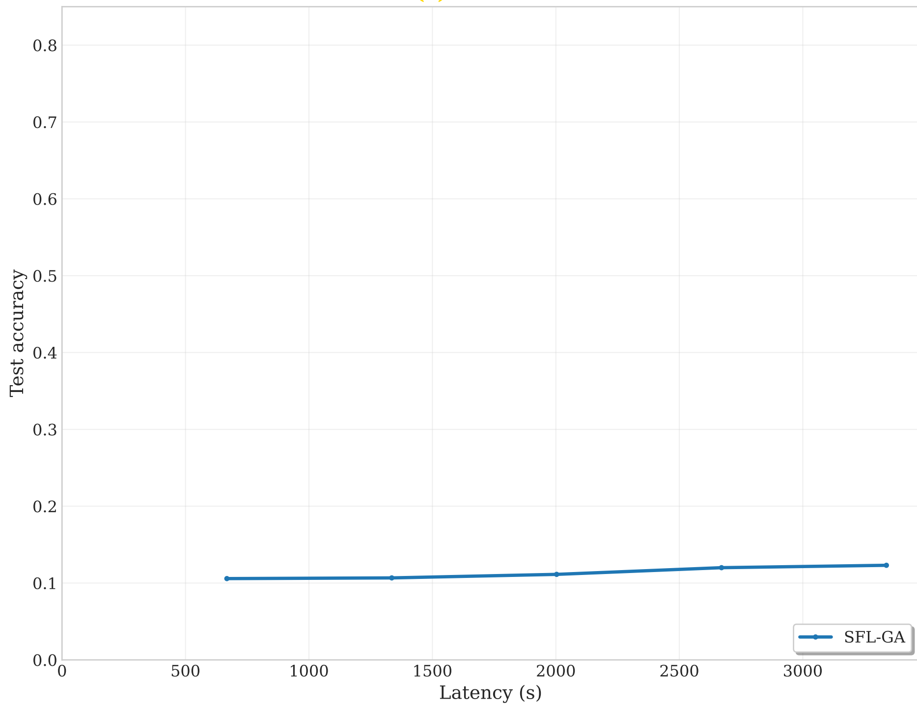
(c) CIFAR-10
