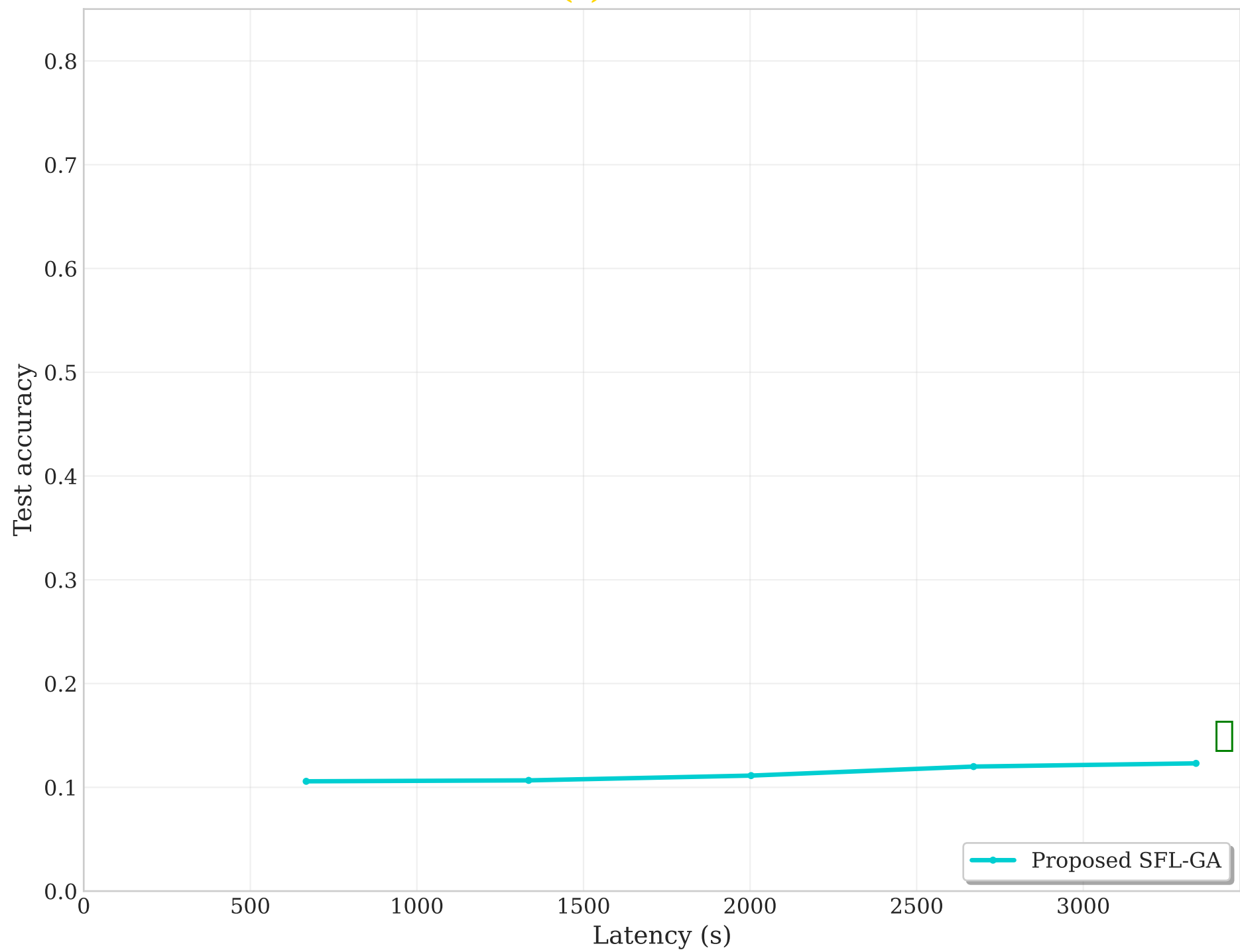
(c) CIFAR-10
