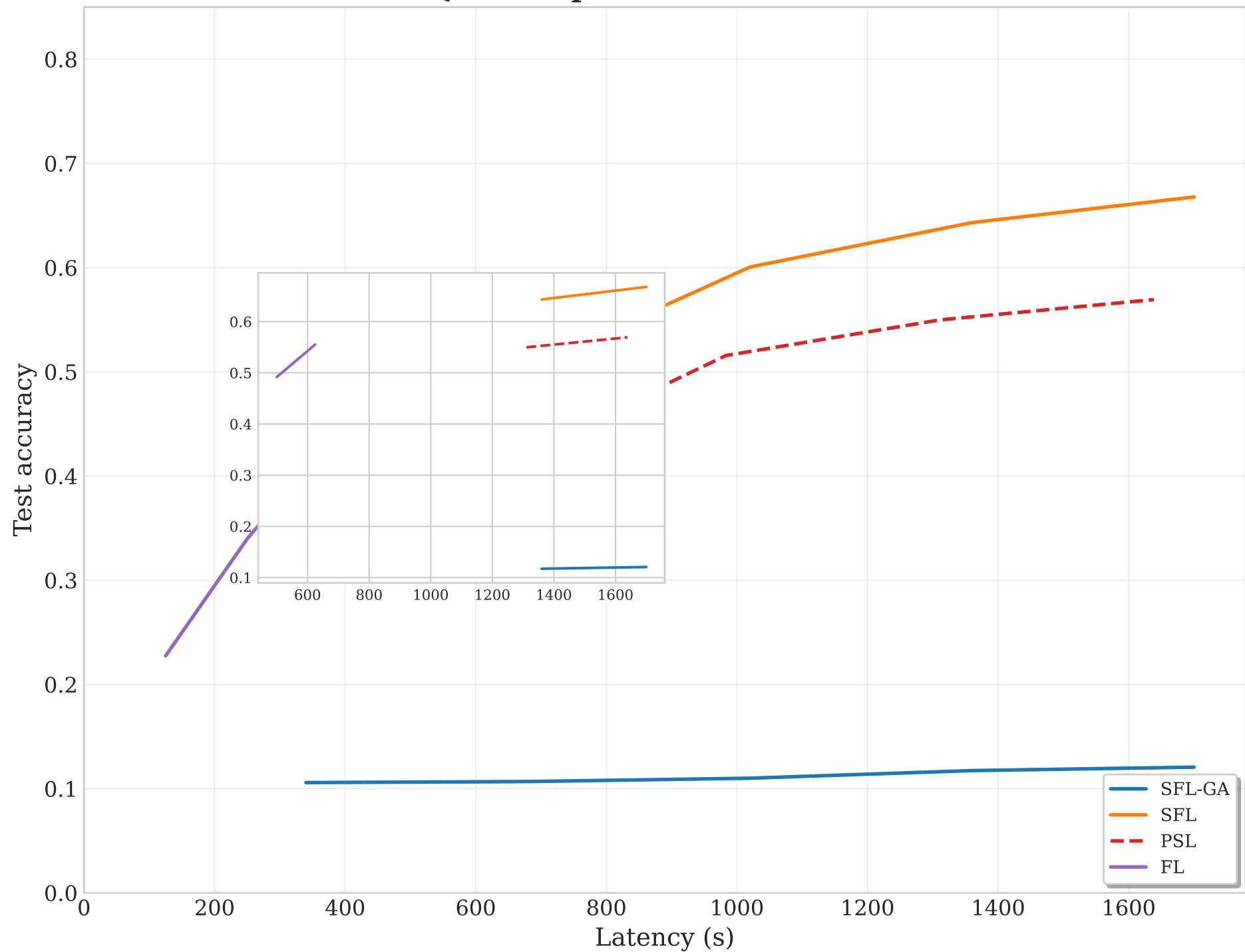
Quick Experiment - CIFAR-10
