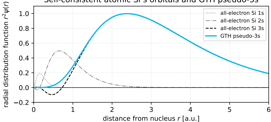
Self-consistent atomic Si s orbitals and GTH pseudo-3s
