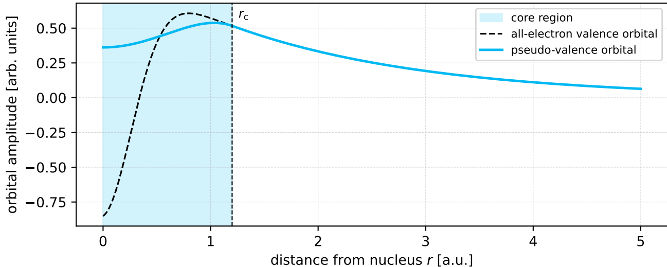
Pseudo-orbital smoothing inside the core region
