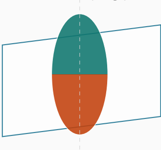
2p_z orbital and sampling plane
