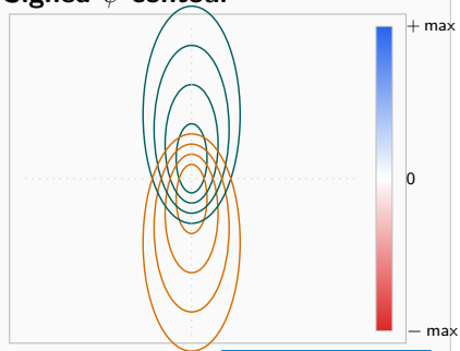
Signed \psi contour
