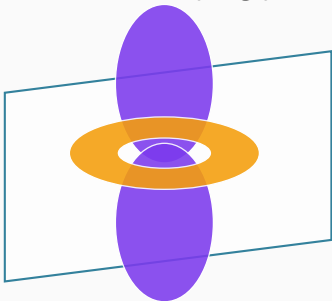
3d_{z^2} orbital and sampling plane
