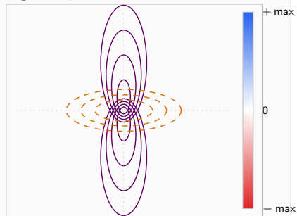
Signed \psi contour
