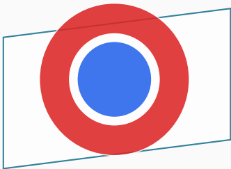
2s orbital and sampling plane
