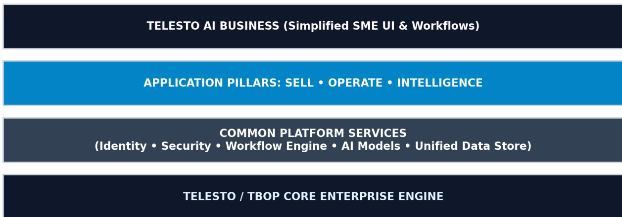
Figure 1: Layered Platform Architecture Stack (TBOP Enterprise Foundation)
