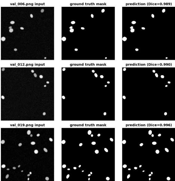
Figure 5: input, ground truth, u-net prediction
