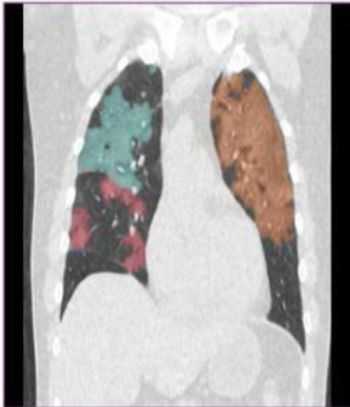
Lobar severity
