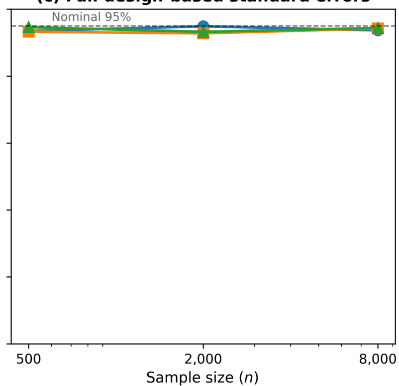
(c) Full design-based standard errors
