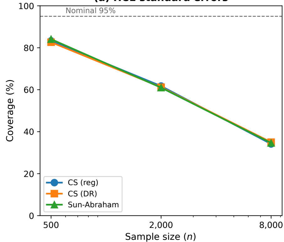
(a) HC1 standard errors
