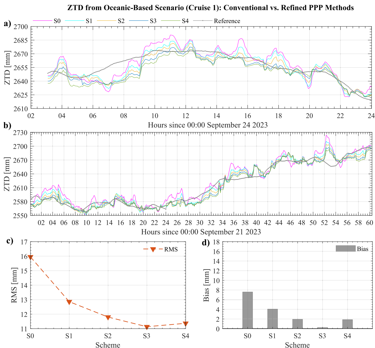
Fig. 8 Time series of ZTD estimated by five schemes during Cruise 1 over two periods: 21 h ( a ) and 60 h, ( b ) starting at 03:00 on September 24, 2023 and 00:00 on September 21, 2023, respectively. Postprocessed
