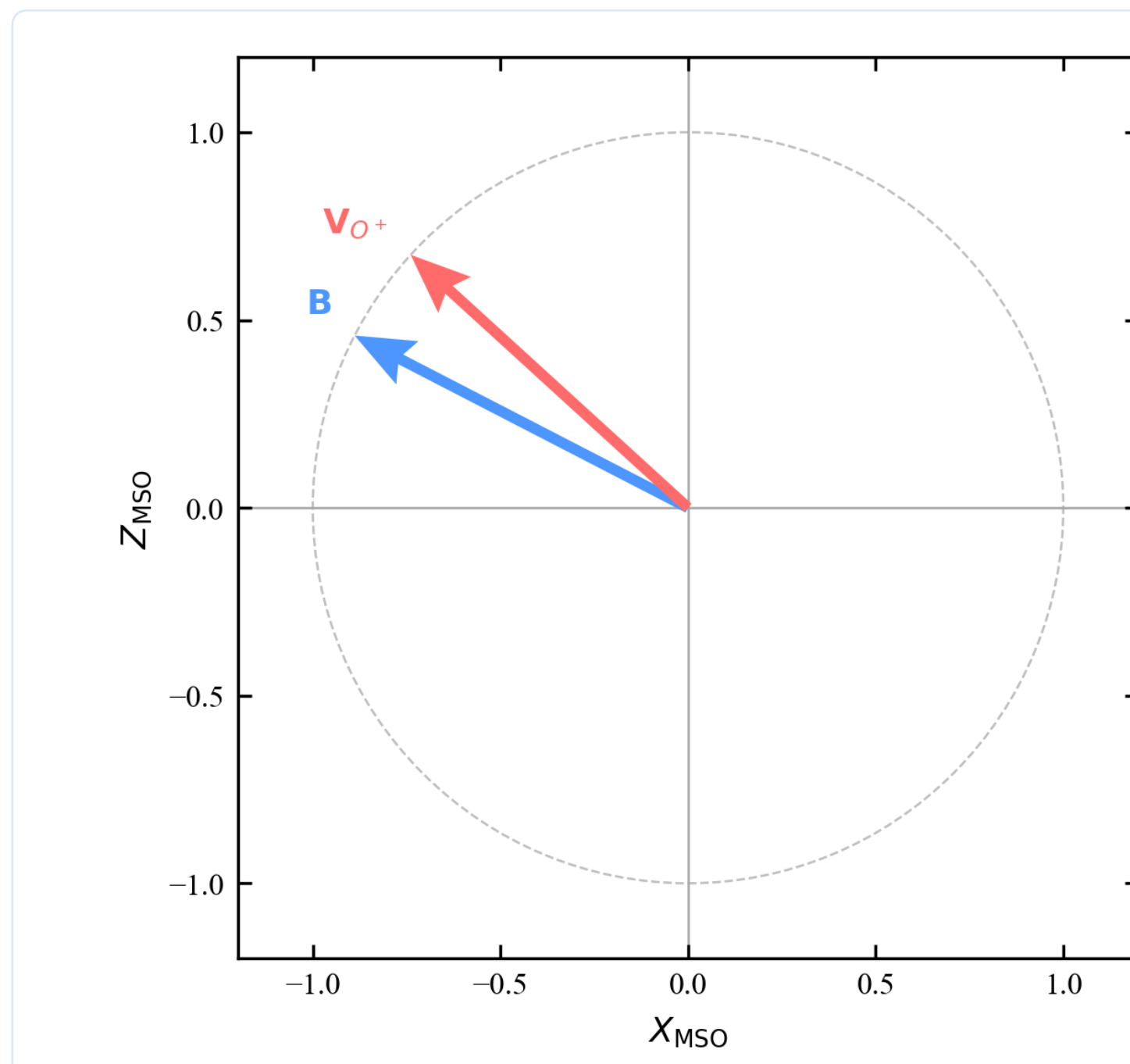
(d) O + Ion Flow and Magnetosheath Magnetic Field Direction in the XZ Plane
