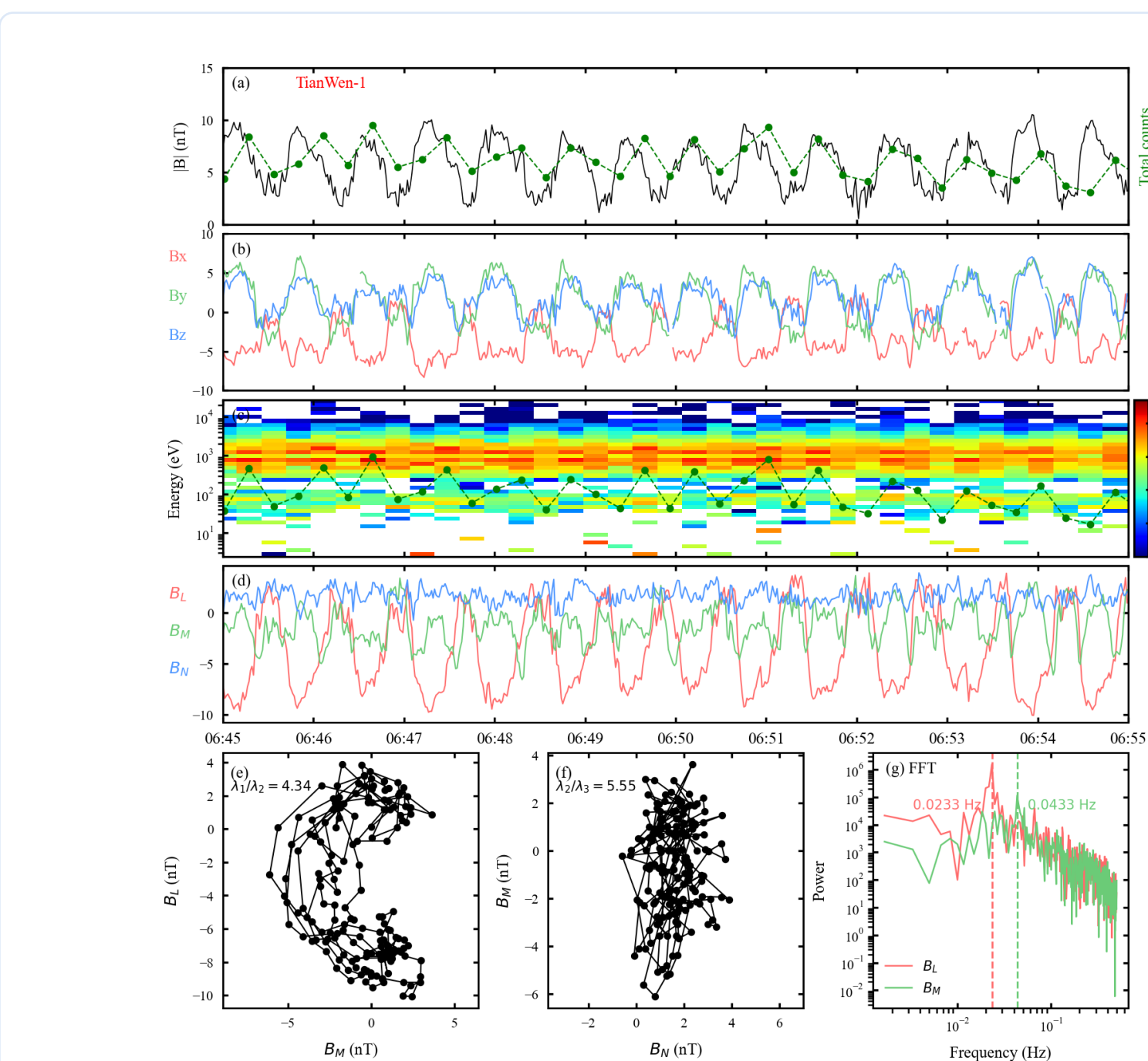
(b) Tianwen-1 observed ~50 s fast-mode waves in magnetosheath.
