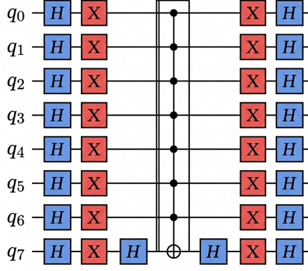
Figure 5. Diffuser for 8 state qubits.
