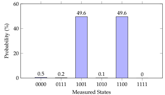
Figure 6. Probability after 8 iterations ( N = 4 ). The two solutions dominate with \sim 49.6\% each; noise < 1\% .
