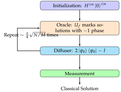
Figure 1. Flow of Grover's algorithm for N-Queens.
