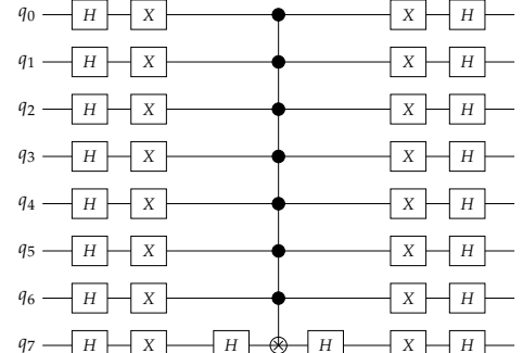
Figure 5. Diffuser circuit for 8 state qubits.
