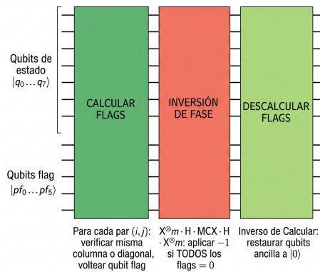
Figura 3. Estructura: Compute \rightarrow Phase Flip \rightarrow Uncompute.
