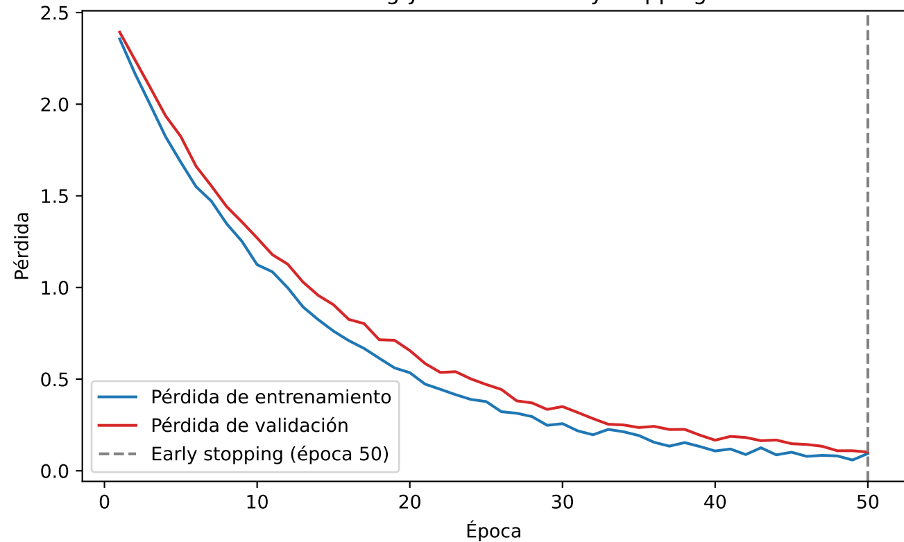
Overfitting y criterio de early stopping
