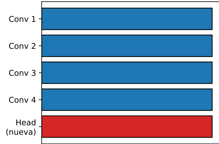
Feature extraction
