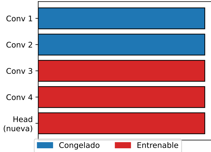
Fine-tuning parcial
