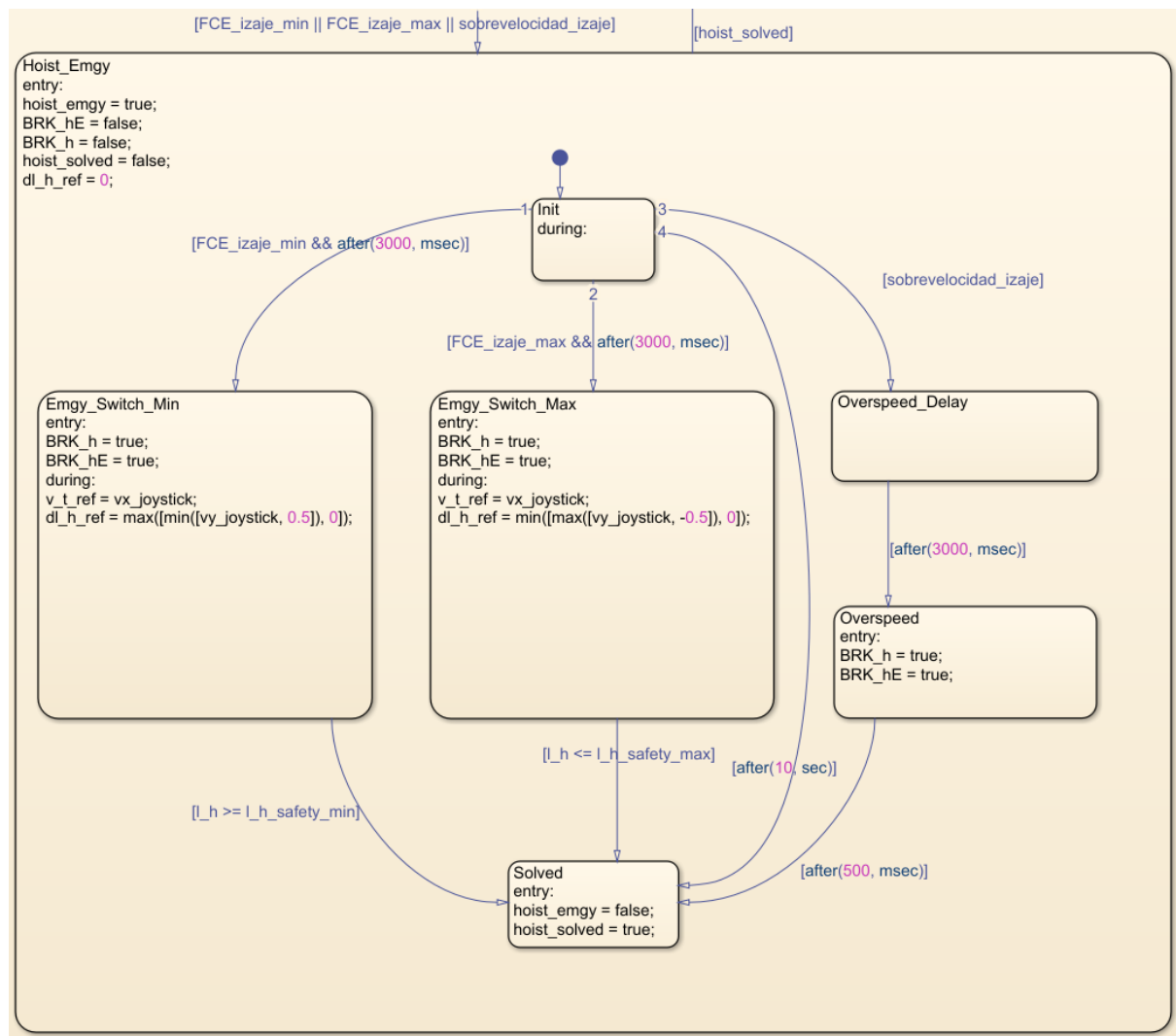
Figura 64: Subestado Hoist_Emg completo: Init, Emgy_Switch_Min, Emgy_Switch_Max, Overspeed_Delay, Overspeed y Solved (Stateflow).
