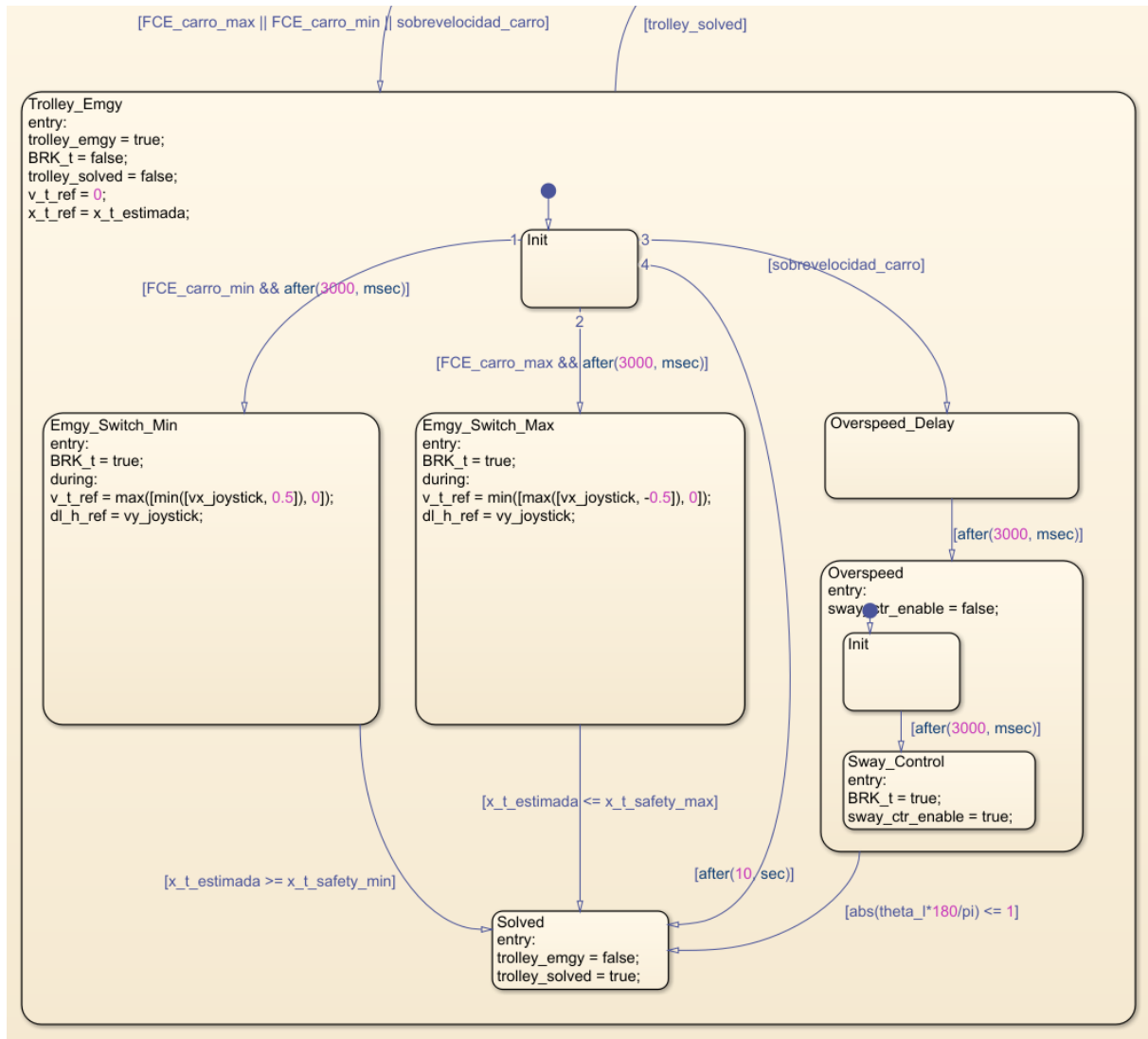
Figura 63: Subestado Trolley_Emg completo: Init, Emgy_Switch_Min, Emgy_Switch_Max, Overspeed_Delay, Overspeed y Solved (Stateflow).
