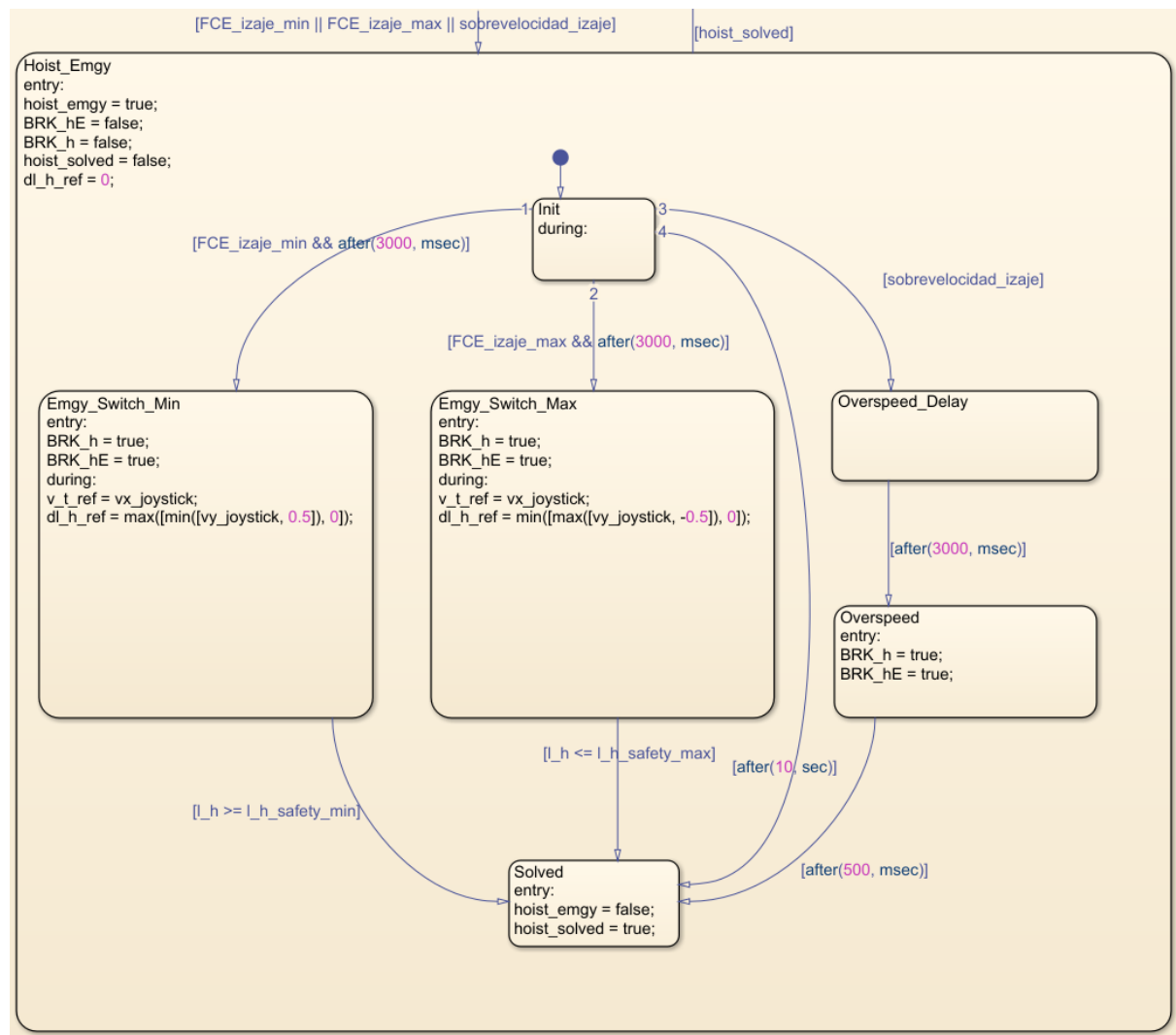
Figura 63: Subestado Hoist_Emg completo: Init, Emgy_Switch_Min, Emgy_Switch_Max, Overspeed_Delay, Overspeed y Solved (Stateflow).
