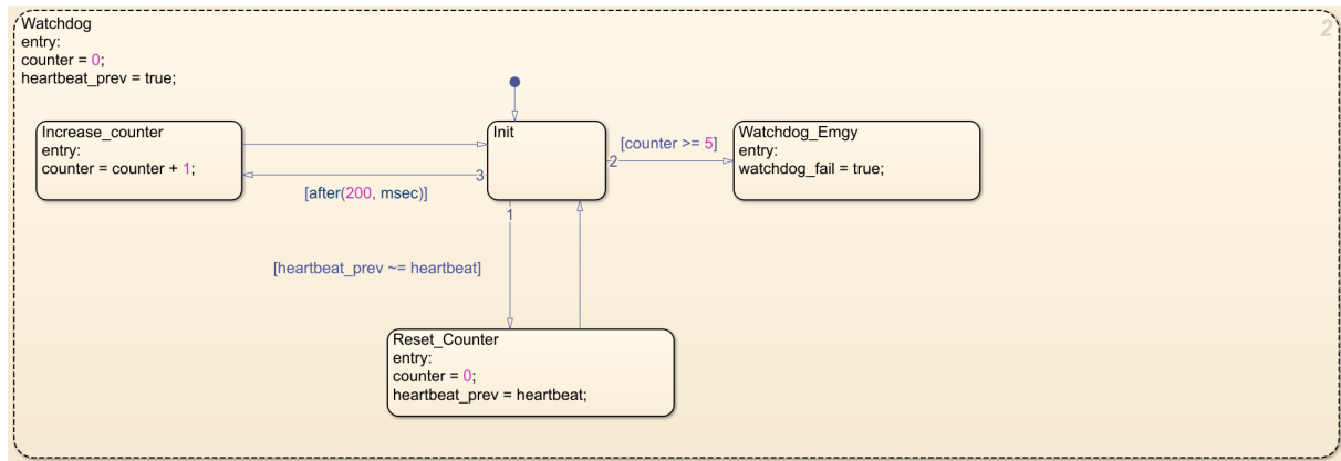
Figura 65: Estado Watchdog completo: Init, Reset_Counter, Increase_counter y Watchdog_Emgy (Stateflow).
