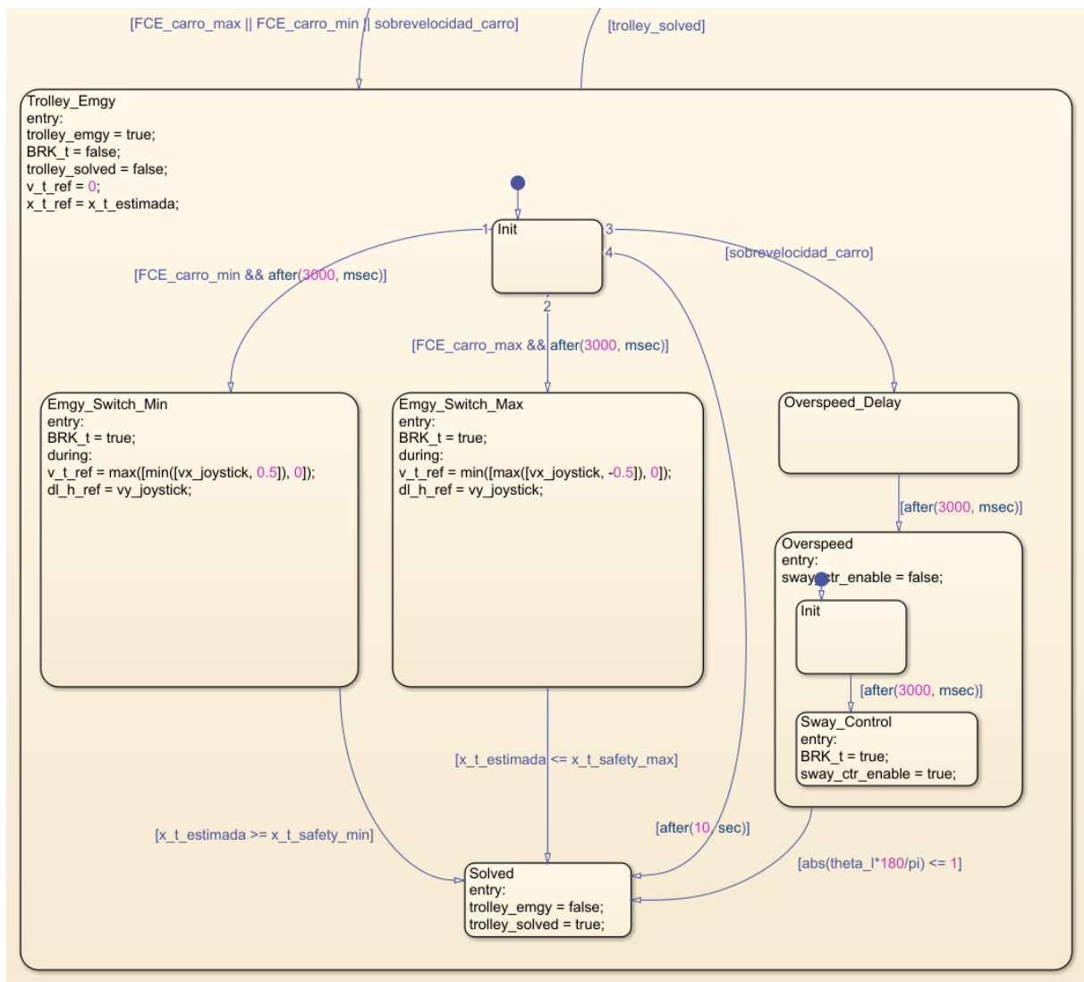
Figura 59: Subestado Trolley_Emg completo: Init, Emgy_Switch_Min, Emgy_Switch_Max, Overspeed_Delay, Overspeed y Solved (Stateflow).
