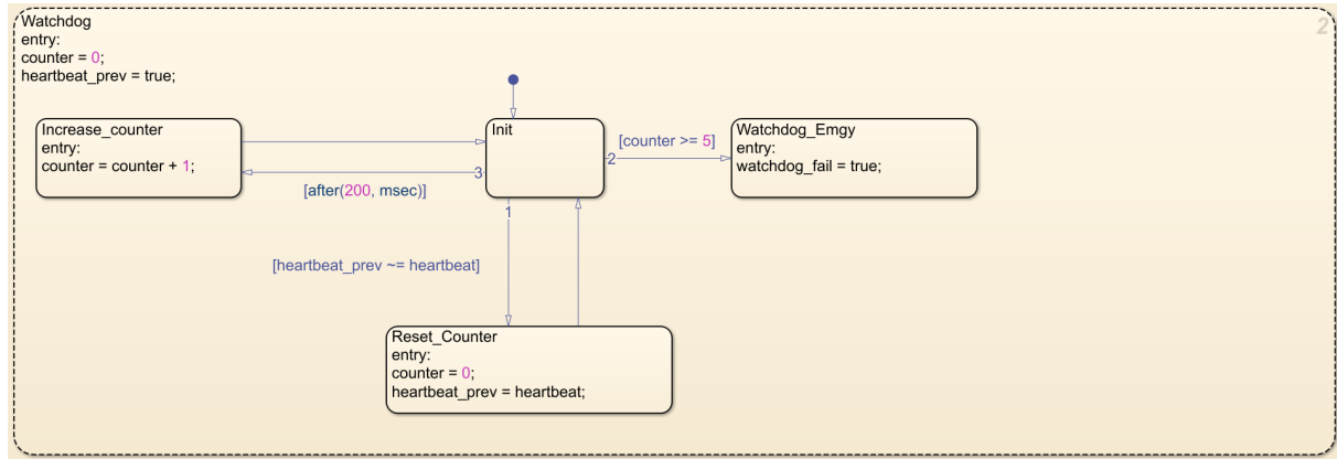
Figura 62: Estado Watchdog completo: Init, Reset_Counter, Increase_counter y Watchdog_Emg (Stateflow).
