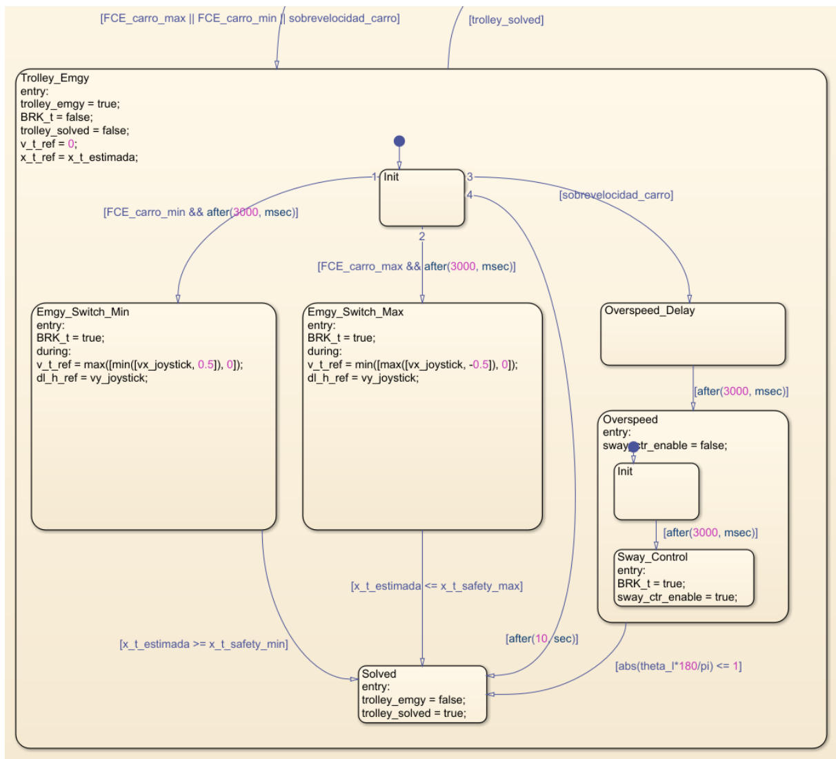
Figura 57: Subestado Trolley_Emg completo: Init, Emgy_Switch_Min, Emgy_Switch_Max, Overspeed_Delay, Overspeed y Solved (Stateflow).
