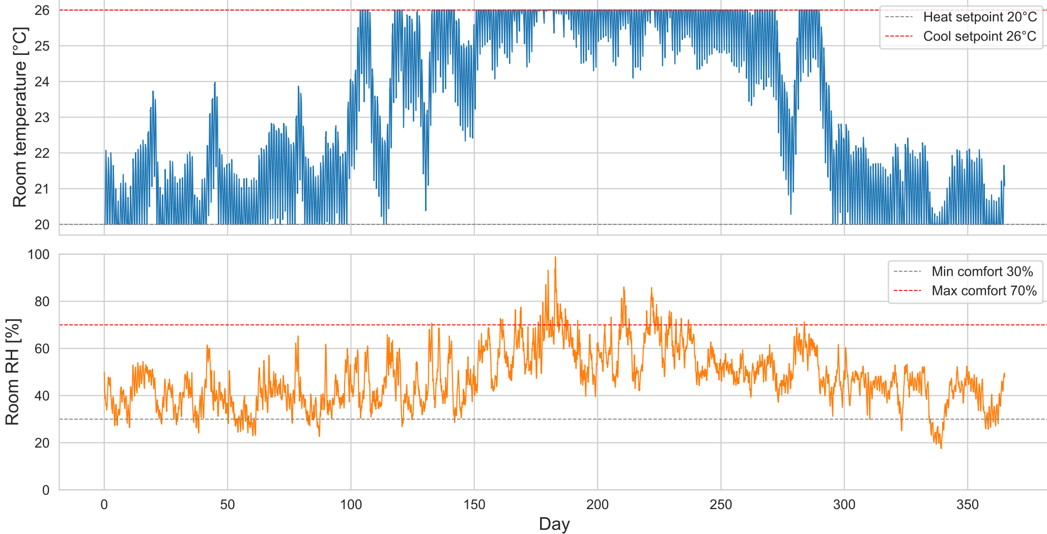
Room thermal & hygric climate — 4 walls
