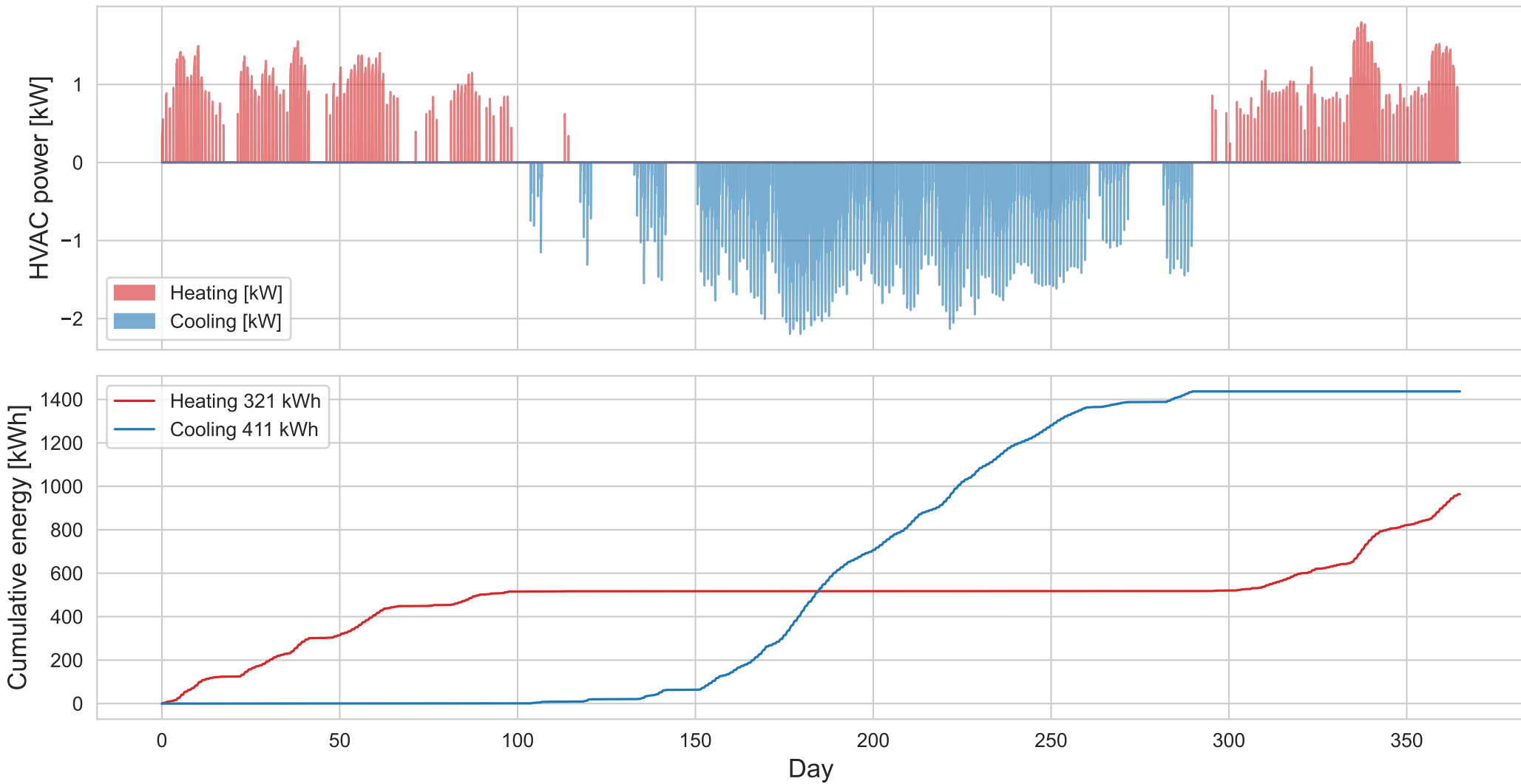
HVAC power and cumulative energy
