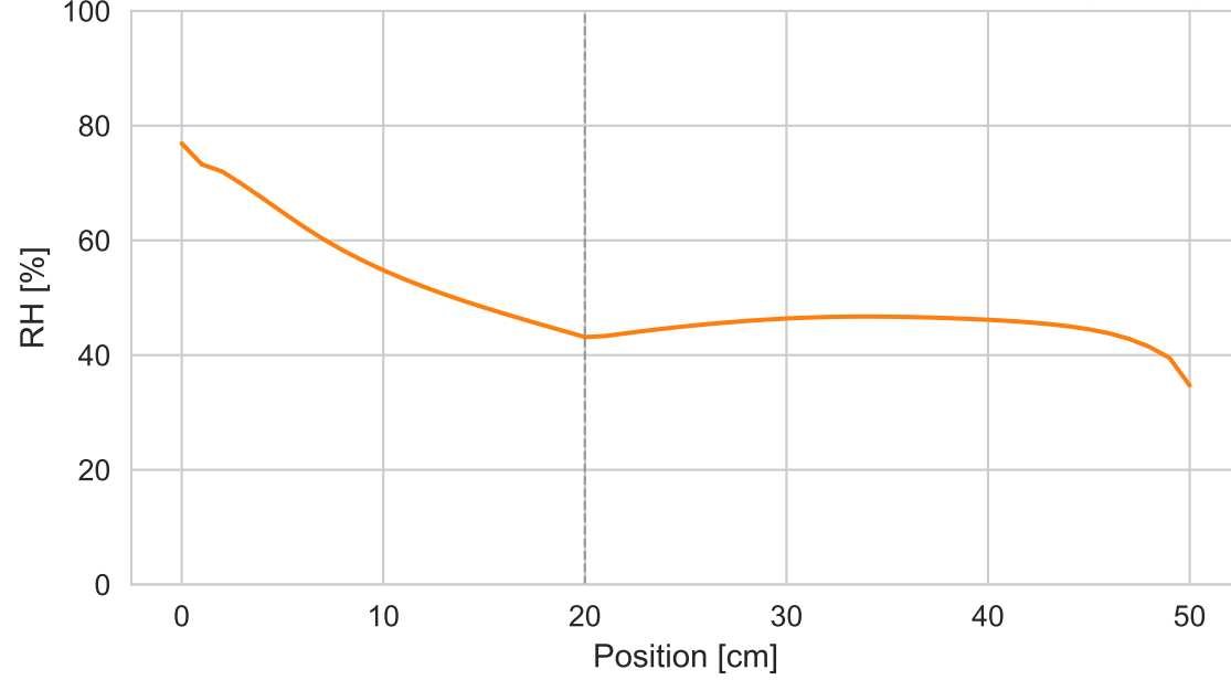
North wall — Concrete + Rock Wool + BA13 — Relative humidity (day 50)
