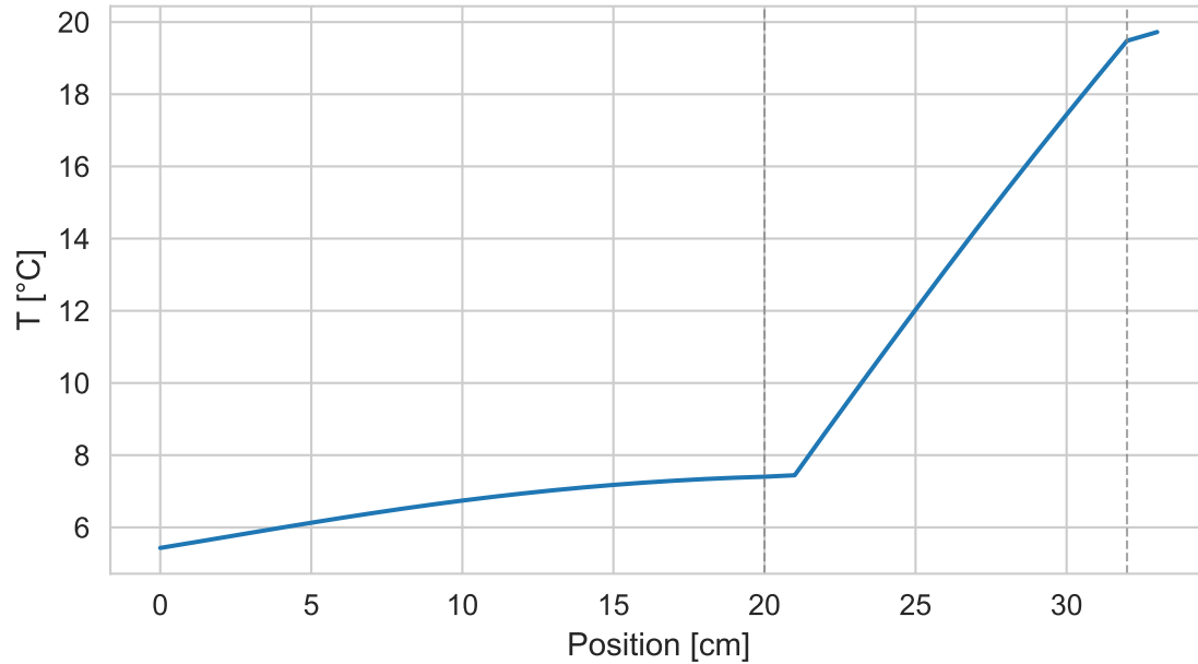
East wall — Wood + Wood Fiber + Fermacell — Temperature (day 50)
