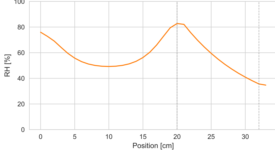
East wall — Wood + Wood Fiber + Fermacell — Relative humidity (day 50)
