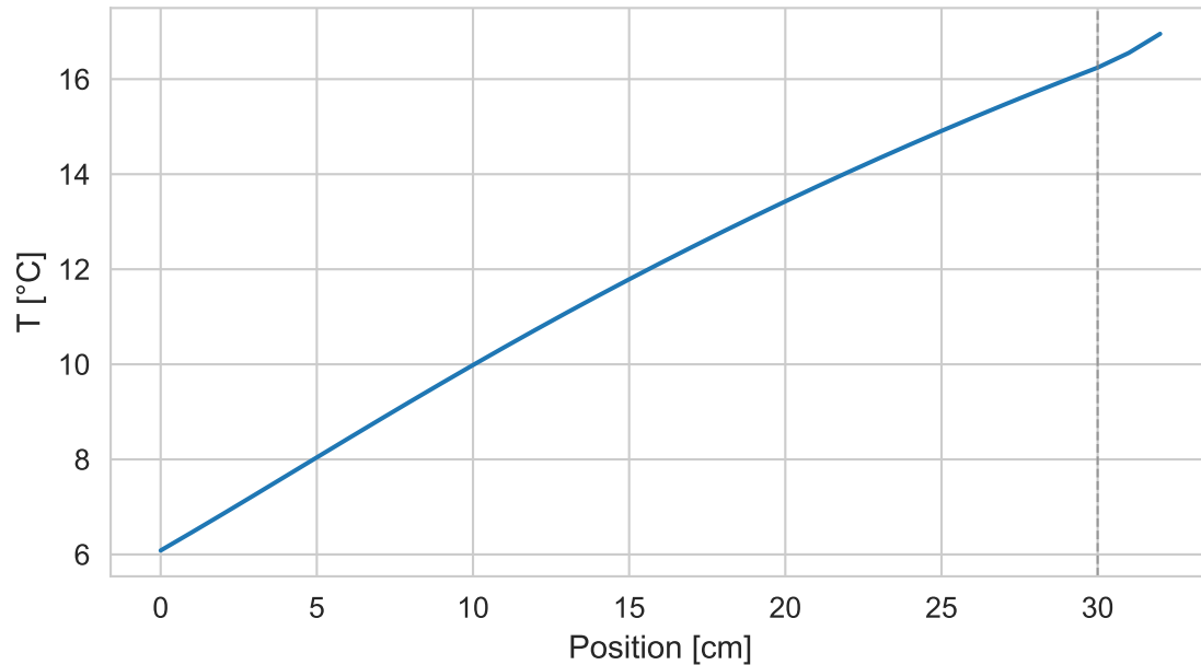
West wall — Rammed Earth + Earth Plaster — Temperature (day 50)
