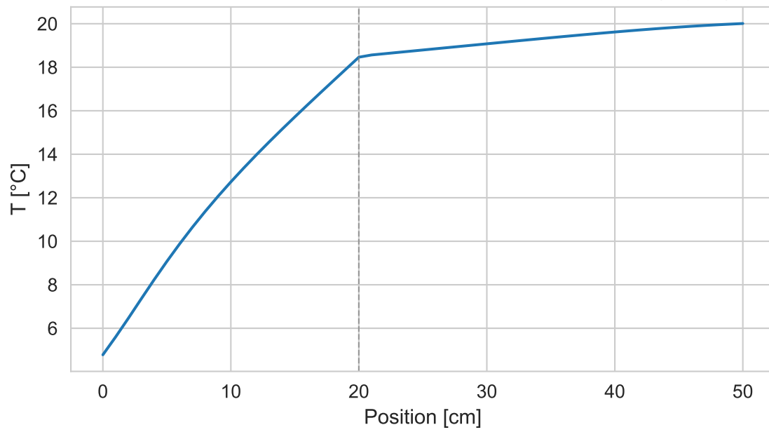
North wall — Concrete + Rock Wool + BA13 — Temperature (day 50)
