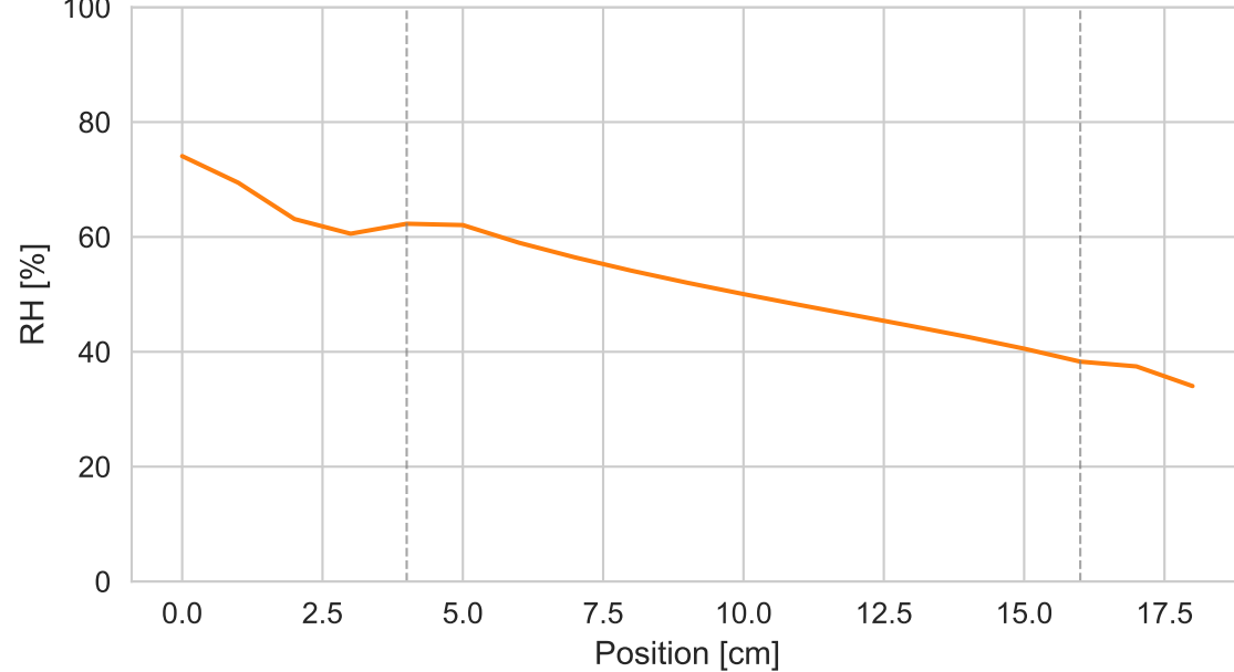
West wall — Rammed Earth + Earth Plaster — Relative humidity (day 50)
