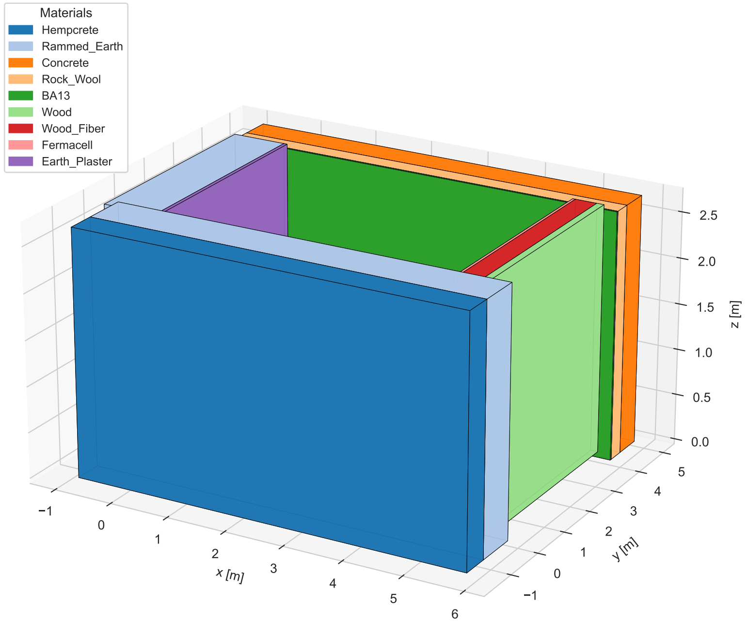
Walls — 3D view (4 walls, layer thickness ×3)
