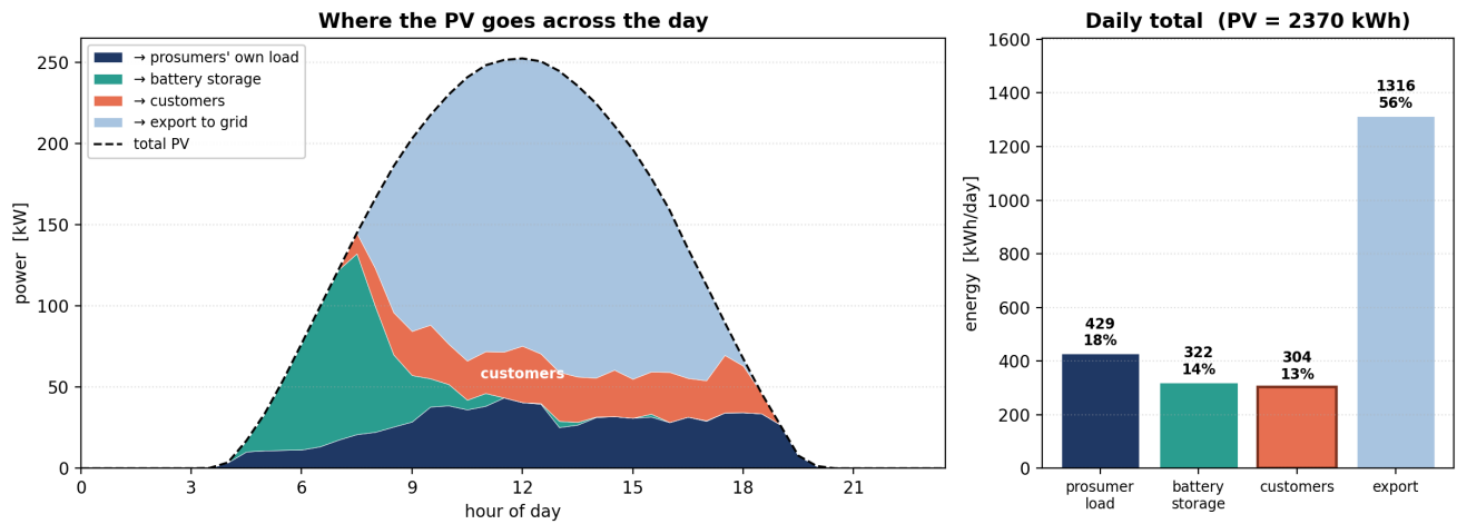
Figure 1: Left: the PV split half-hour by half-hour. In the early morning the batteries absorb the surplus; once they fill up (late morning) the surplus goes to customers and export. Right: daily totals.
