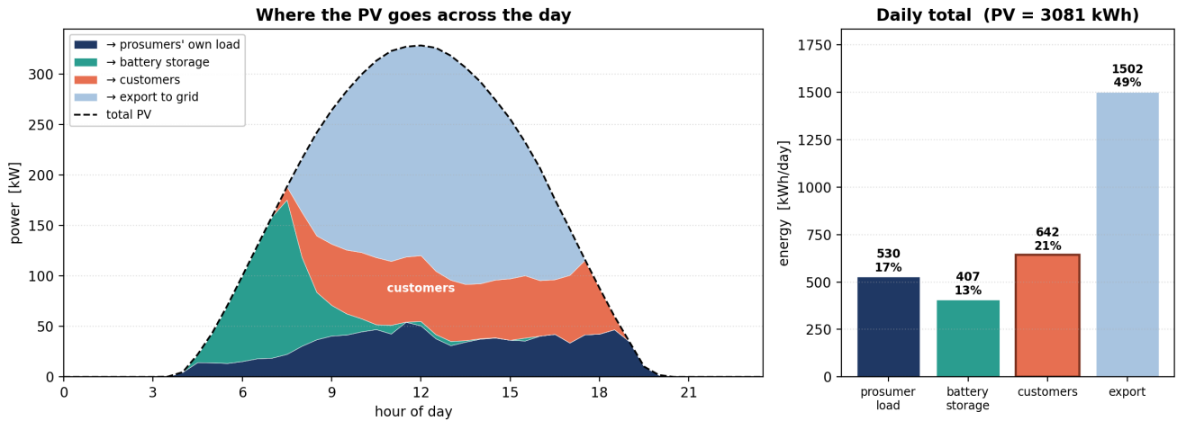
Figure 1: Left: the PV split half-hour by half-hour. In the early morning the batteries absorb the surplus; once they fill up (mid-morning) the surplus goes to customers and export. Right: daily totals.
