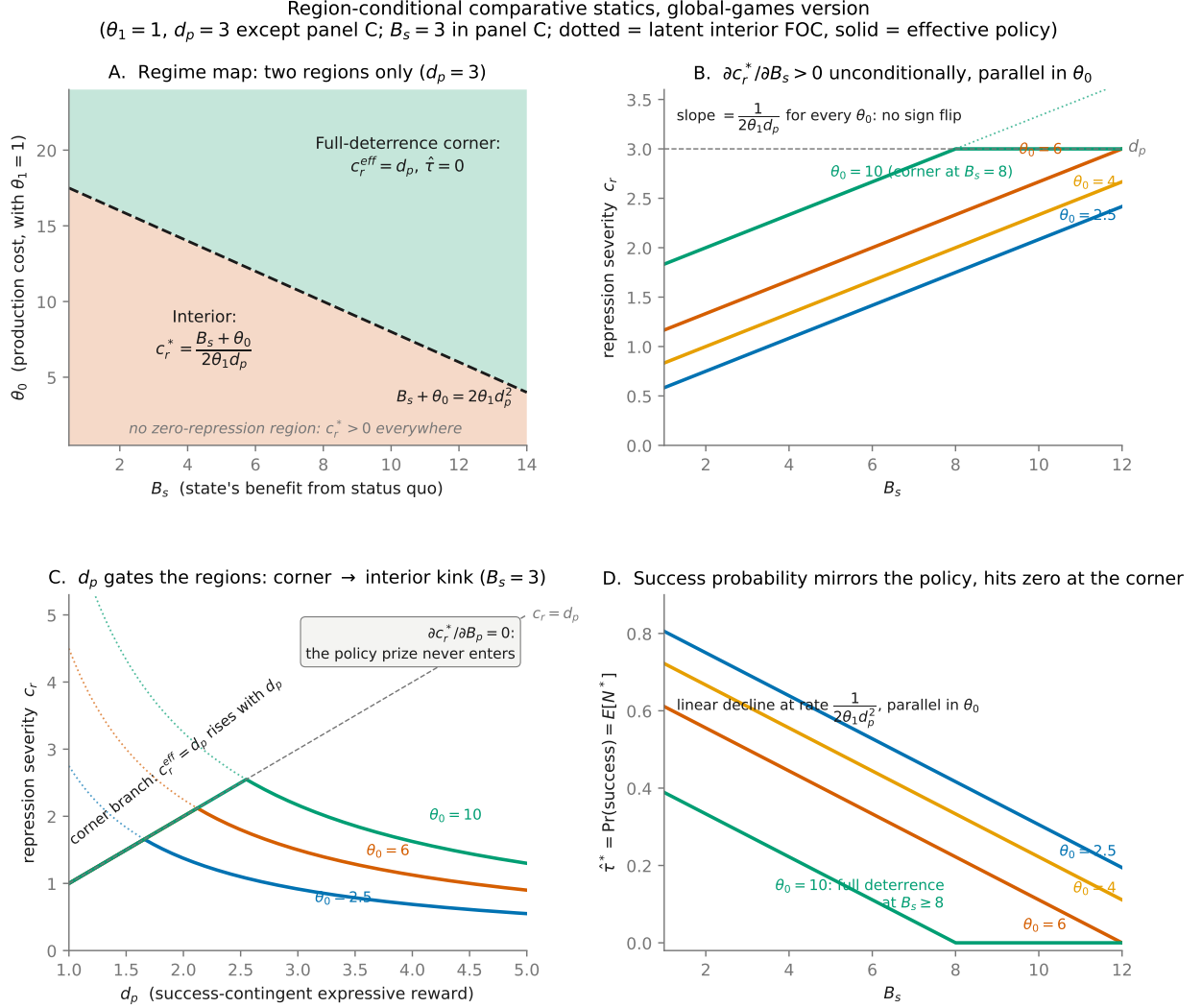
Figure 1: Region-conditional comparative statics of the repression severity policy ( \theta_1 = 1 ; d_p = 3 except in panel C; B_s = 3 in panel C). Panel A maps the two regions of the parameter space: the interior solution and the full-deterrence corner, separated by B_s + \theta_0 = 2\theta_1 d_p^2 ; there is no zero-repression region. Panel B shows that c_r^* rises linearly in B_s with slope 1/(2\theta_1 d_p) for every \theta_0 , flattening at the corner c_r = d_p . Panel C shows the kinked, non-monotone effect of d_p : the effective policy rides the corner c_r = d_p upward while full deterrence is cheap, then switches to the declining interior solution. Panel D plots the equilibrium success probability \hat{\tau}^* , which declines linearly in B_s at rate 1/(2\theta_1 d_p^2) and reaches zero at the corner. Dotted curves are the latent interior first order condition; solid curves are the effective policy.
