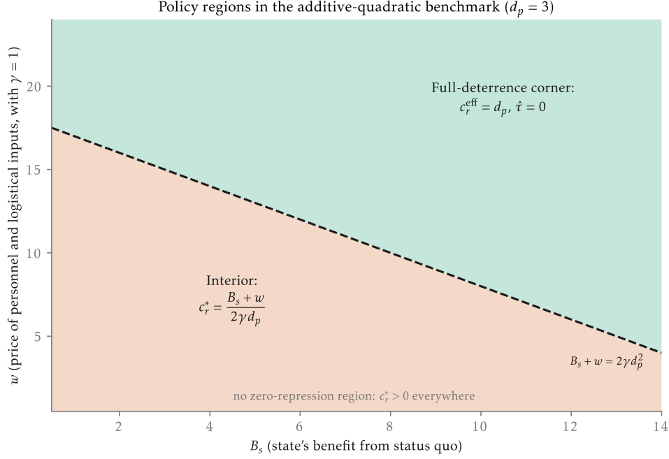
Figure A1: Interior and full-deterrence regions for V(\bar{N}, c_r; w) = w\bar{N} and P(c_r; \gamma) = \gamma c_r^2 . The boundary is B_s + w = 2\gamma d_p^2 .
