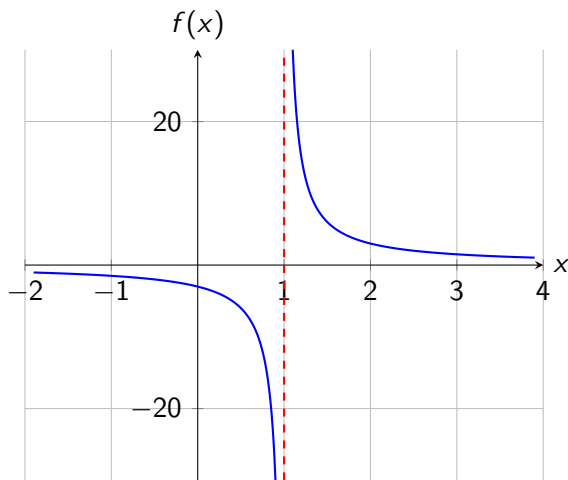
Figure: f(x) = \frac{3}{x-1} , with the vertical asymptote at x = 1 dashed. The two branches are drawn separately because the function is undefined there.
