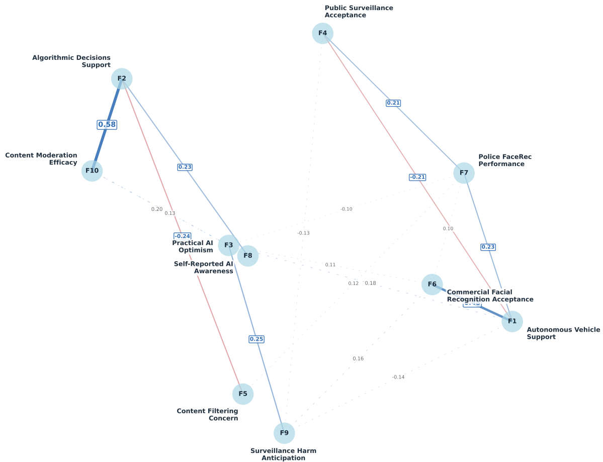
Partial-Correlation Network (10 factors, |p| \geq 0.10 )
