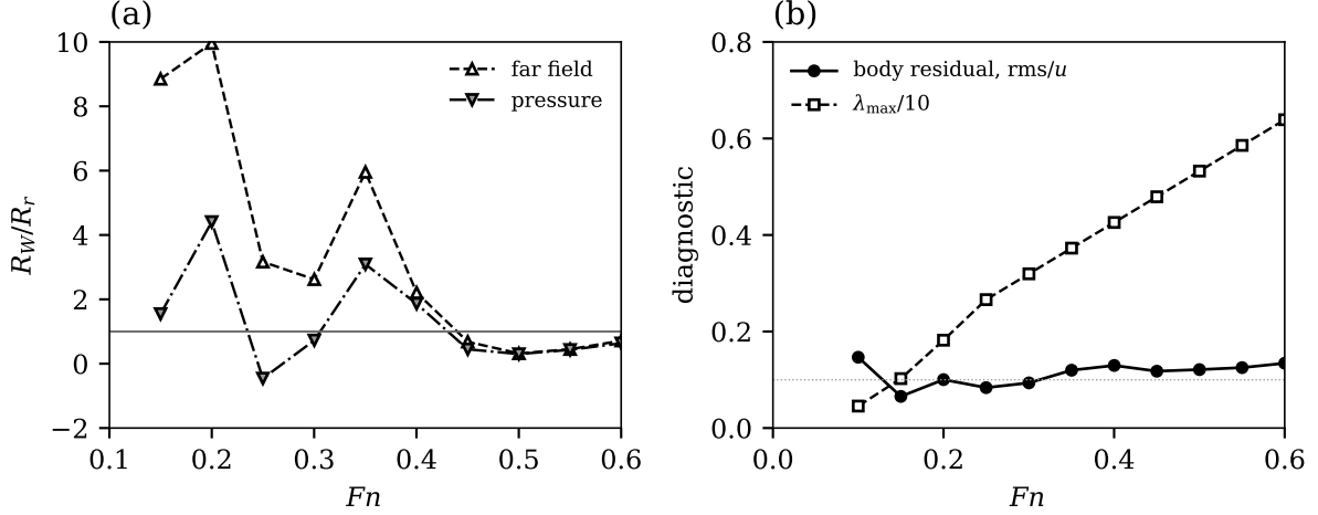
Figure 4: Diagnostics versus Fn for Sysser 01 on the 280-panel mesh at the static attitude: (a) ratio of predicted wave resistance to measured residuary resistance by both routes, plotted where R_r exceeds 0.05 N, with the dark line marking unity; (b) root-mean-square body-condition residual at points that are not collocation points, as a fraction of u , and the largest wave parameter the mesh resolves, divided by ten to share the ordinate. The dotted line marks a residual of 0.1.
