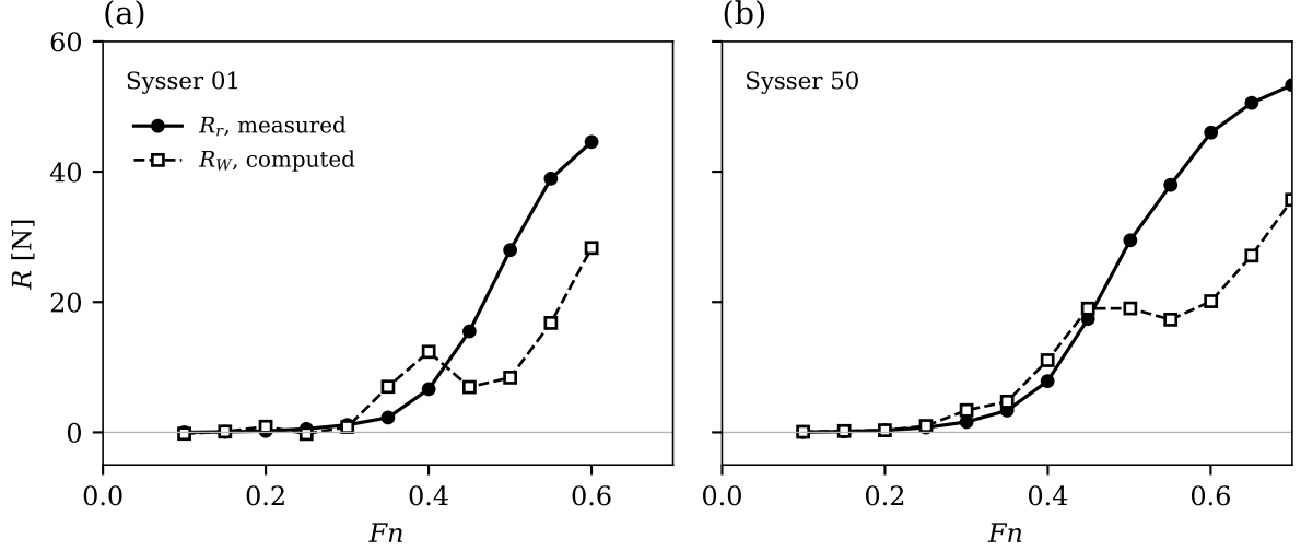
Figure 7: Computed wave resistance and measured residuary resistance versus Fn for (a) Sysser 01 on a 280-panel mesh and (b) Sysser 50 on a 320-panel mesh, both at the static attitude and both by the pressure route. Residuary resistance is a proxy for wave resistance rather than a measurement of it: it follows from the measured total resistance by subtracting an ITTC-57 friction line at form factor zero, so it also contains nonlinear and viscous-form contributions.
