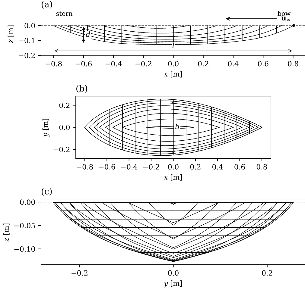
Figure 1: Wetted surface of Sysser 01 at the reference condition, with the waterline length l , the waterline beam b , the canoe-body draught d , and the onset flow \mathbf{u}_\infty : (a) buttock lines and stations in profile, (b) waterlines in plan, (c) stations and waterlines in the body plan. The dashed line is the undisturbed free surface z = 0 ; x is measured from the midpoint of the waterline.
