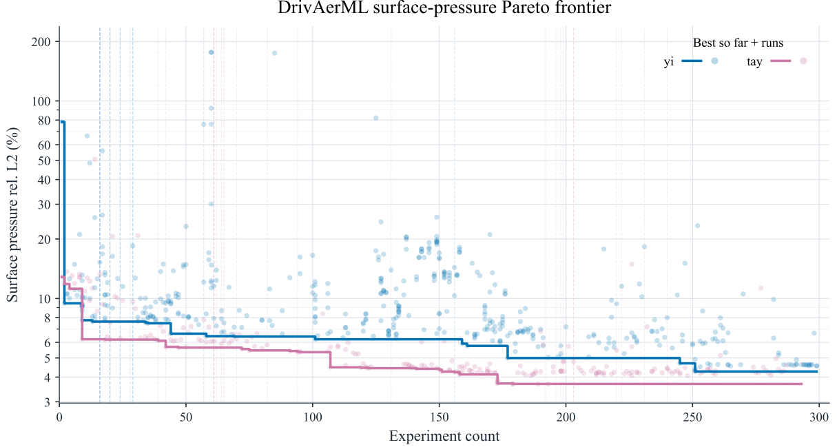
Figure 4. Evolution of DrivAerML surface-pressure test error across two SENPAI campaigns. Faded markers show individual completed experiments from the yi and tay branches, while solid curves show the cumulative Pareto frontier: the best surface-pressure relative L_2 error achieved up to each experiment count. The vertical lines mark GitHub-recorded human researcher/operator interventions. tay was instructed to use DDP8 and was given a 6 hour per-experiment training budget, hence the better performance.
