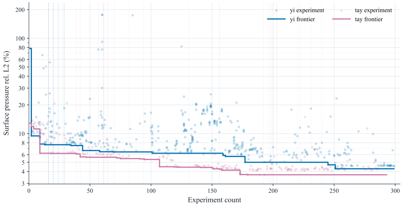
DrivAerML surface-pressure Pareto frontier
