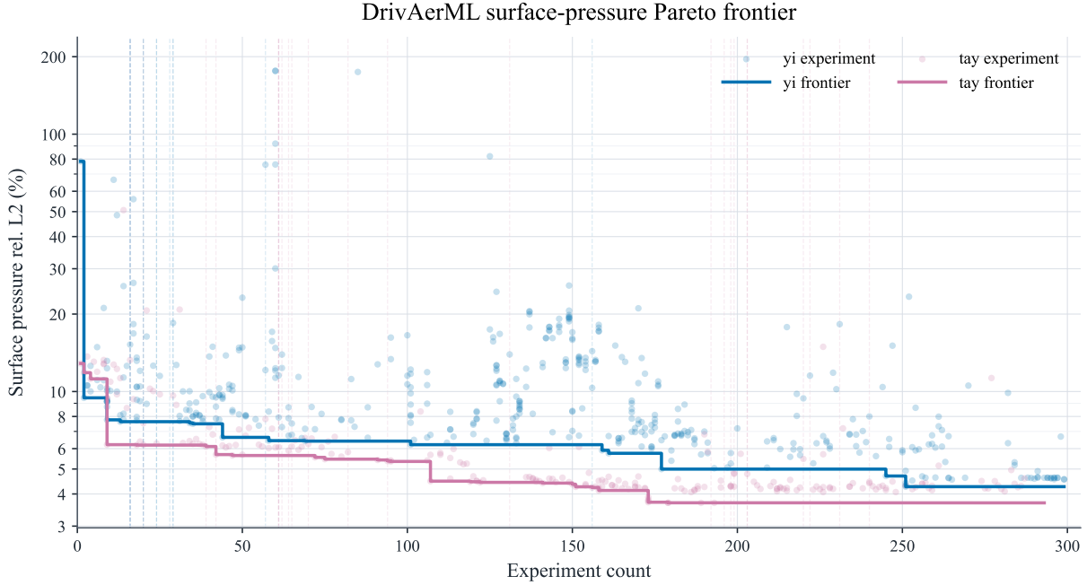
Figure 2. Evolution of DrivAerML surface-pressure test error across two SENPAI campaigns. Faded markers show individual completed experiments from the yi and tay branches, while solid curves show the cumulative Pareto frontier: the best surface-pressure relative L_2 error achieved up to each experiment count. The vertical lines mark GitHub-recorded human researcher/operator interventions. tay was instructed to use DDP8 and was given a 6 hour per-experiment training budget, hence the better performance.
