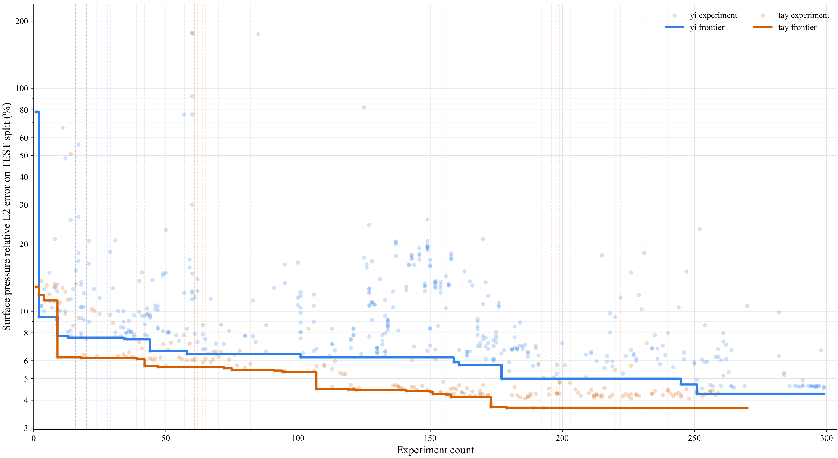
DrivAerML surface-pressure test Pareto frontier
