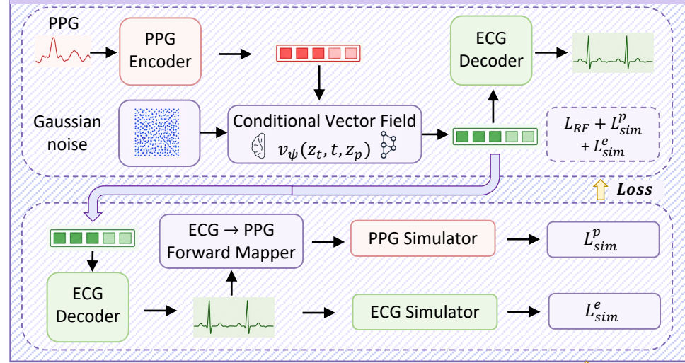
(c) Electro-Hemodynamic Simulator Guided Latent Rectified Flow
