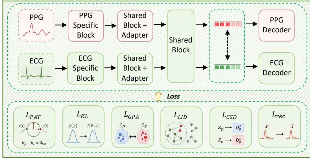
(b) Physiology-Aware AutoEncoder
