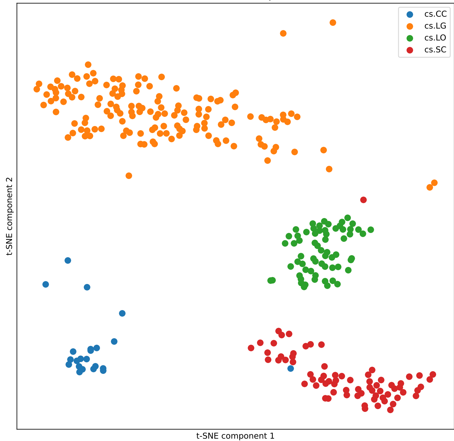
t-SNE Visualization by Label
