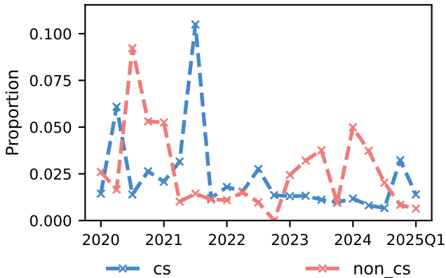
Cpp File - camelCase
