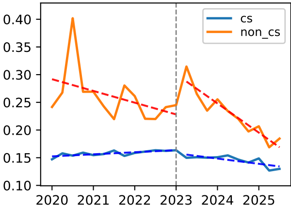
Estimated Bugs
