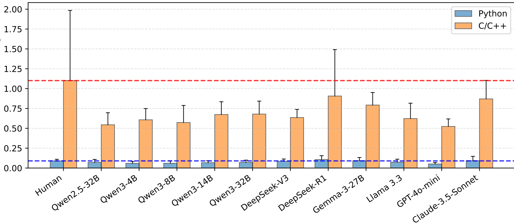
Halstead Estimated Bugs
