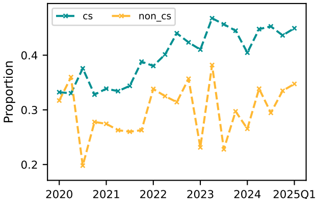
cpp Function Names - snake_case
