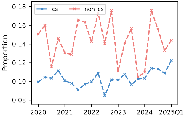
cpp Variable Names - single_letter
