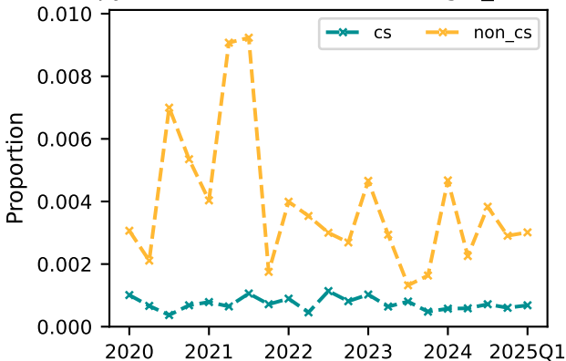
python Function Names - single_letter
