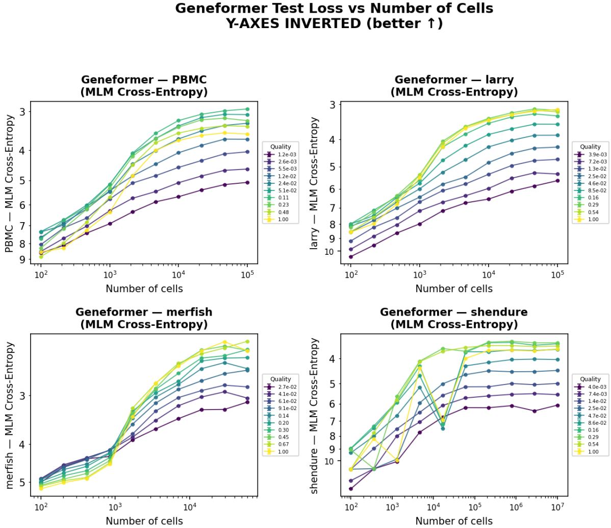
Figure 1: Geneformer final test loss vs. training-set size on a log-log scale, one curve per quality level.
