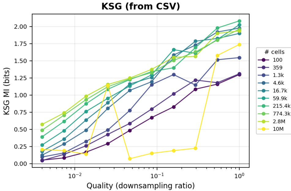
Figure 5: KSG MI (bits) for SCVI on shendure vs. measurement quality (log scale), one curve per dataset size.
