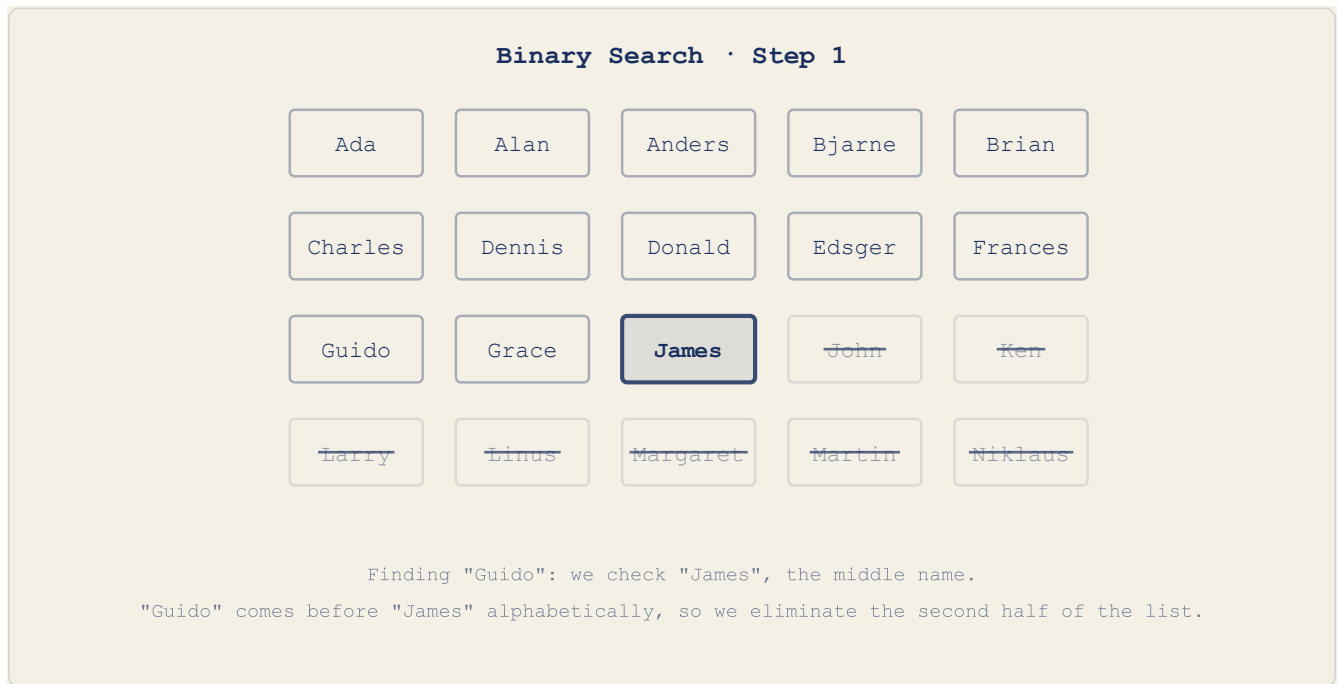
Figure 1.2: Binary Search Step 1
