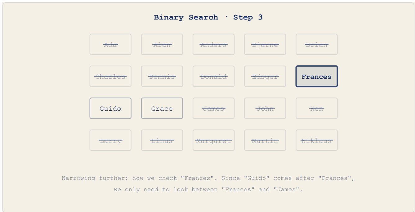
Figure 1.4: Binary Search Step 3
