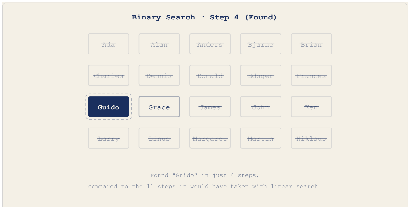
Figure 1.5: Binary Search Step 4
