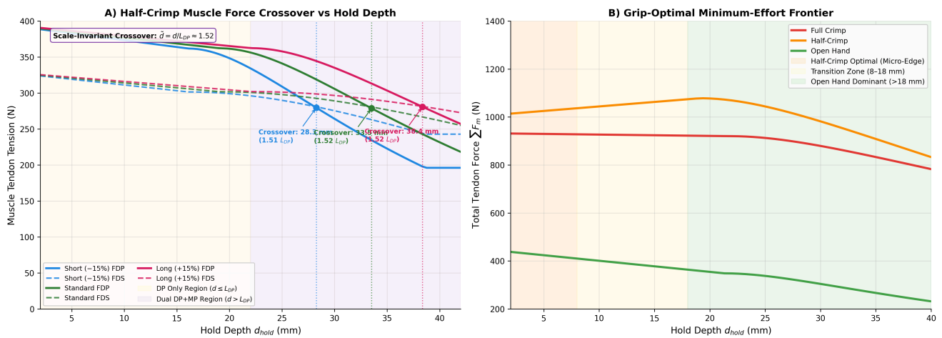
Figure 2: Hold depth force redistribution and grip optimization. (A) Muscle tendon forces (FDP: solid, FDS: dashed) across hold depths ( d_{hold} \in [2, 42 mm]) in Half-Crimp for Short (−15%, blue), Standard (green), and Long (+15%, magenta) phenotypes. Crossover points where FDS surpasses FDP as prime mover occur at 28.3 mm (Short), 33.5 mm (Standard), and 38.4 mm (Long), all corresponding to a scale-invariant dimensionless hold depth \tilde{d} = d/L_{DP} \approx 1.52 . Yellow background shading indicates the single-segment DP region ( d \leq L_{DP} ); purple shading indicates dual DP+MP contact. (B) Minimum-effort energetic grip frontier showing total tendon force across hold depths, with shaded background zones indicating optimal grip selection: Half-Crimp ( < 8 mm, orange), Transition Zone (8–18 mm, yellow), and Open Hand ( > 18 mm, green).
