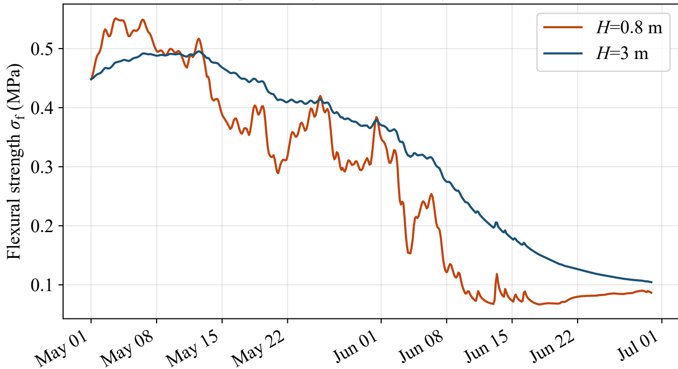
Depth-averaged flexural strength vs. time
