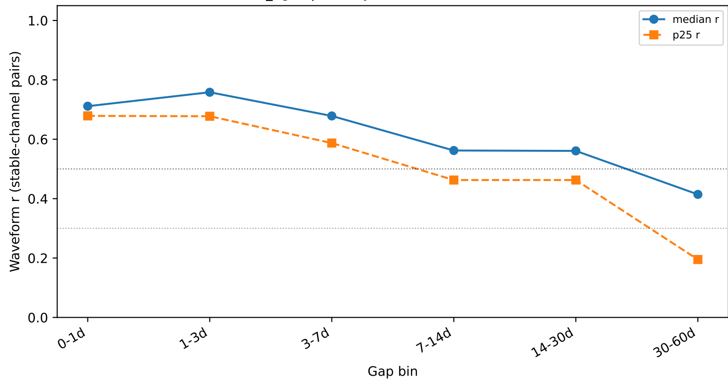
Curius_AgoB | stability across sessions (stable n=6)
